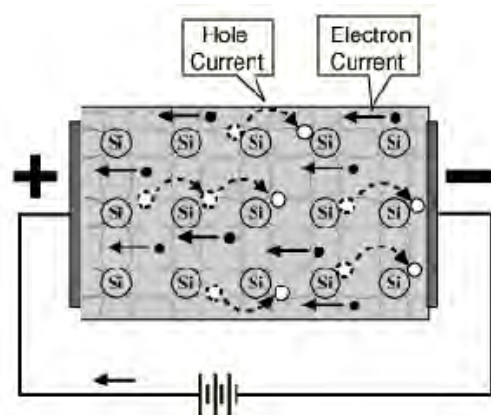
Figure 3. Schematic of the electrical conduction through a semiconductor material driven by a battery. Holes and electrons both contribute to electrical conduction.
